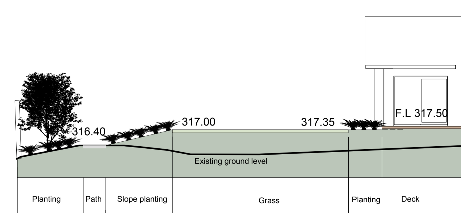
1 Indicative Cross Section AA 1:100
